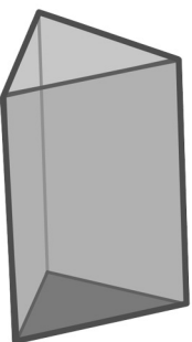
Triangular Prism
