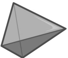
Triangular Pyramid
