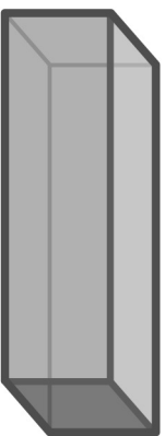
Rectangular Prism
